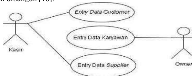
Gambar 3. Use Case Diagram Master Jeviya Beauty Bar
